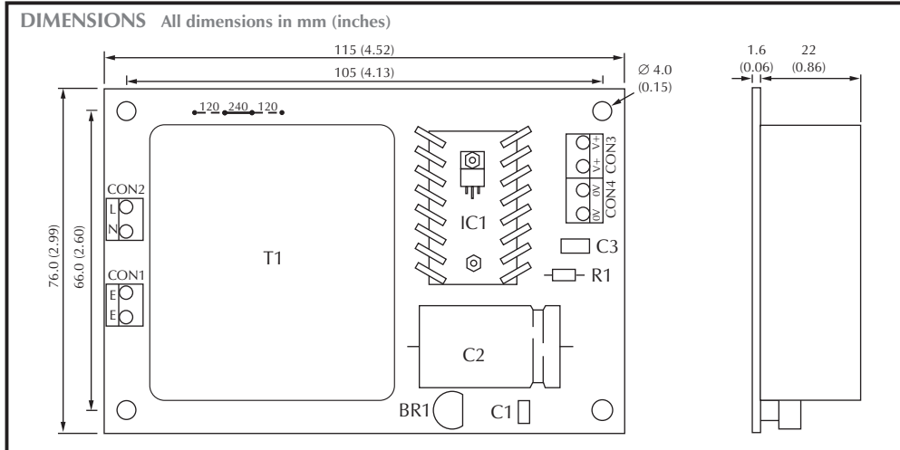
Specifications liable to change without prior warning PSU 201 Issue 12 09/2010 S.L. Applies to PSU 201/4
